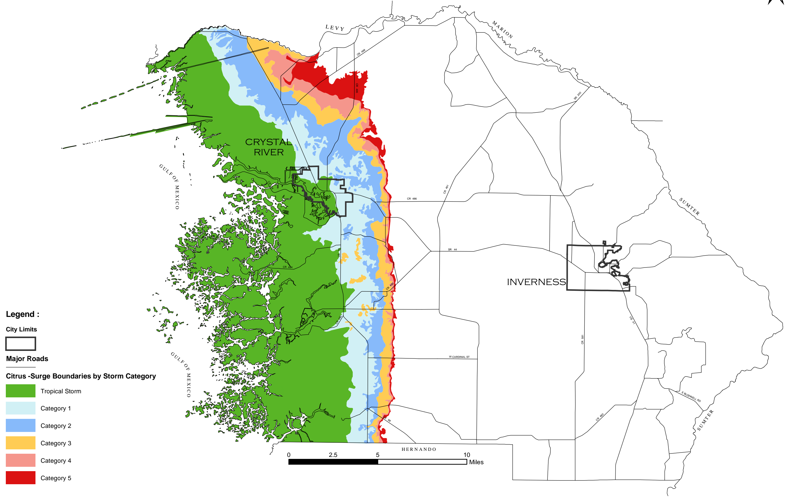
MAP 3 Citrus County Maximum of Maximum Inland Surge Boundary - SLOSH Model Data
